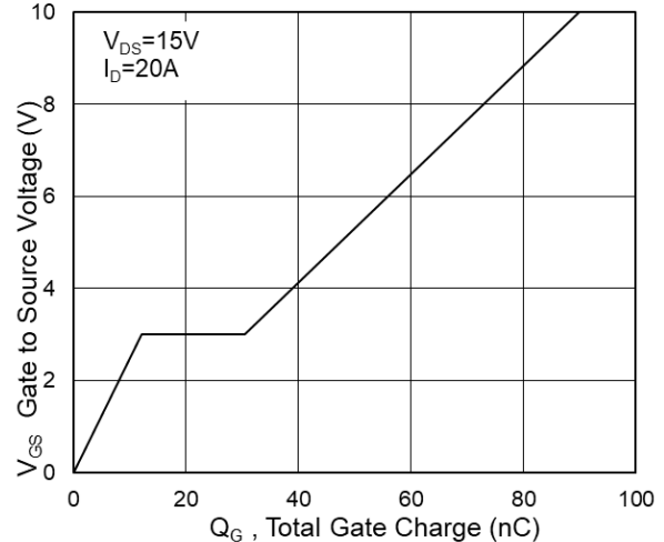
Fig.6 Gate-Charge Characteristics
